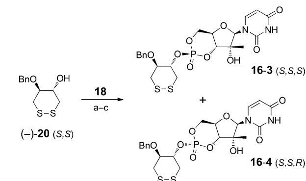
Scheme 6. Synthesis of cyclic-disulfide-based prodrugs 16 . Reaction conditions: a) ethylthiotetrazole, MeCN; b) t\text{BuOOH} , MeCN; c) preparative HPLC separation. Bn = benzyl.
